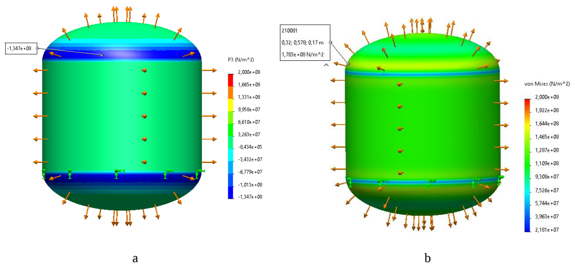
Figure 4. Distribution of circular – a and equivalent – b stresses in the bottom
